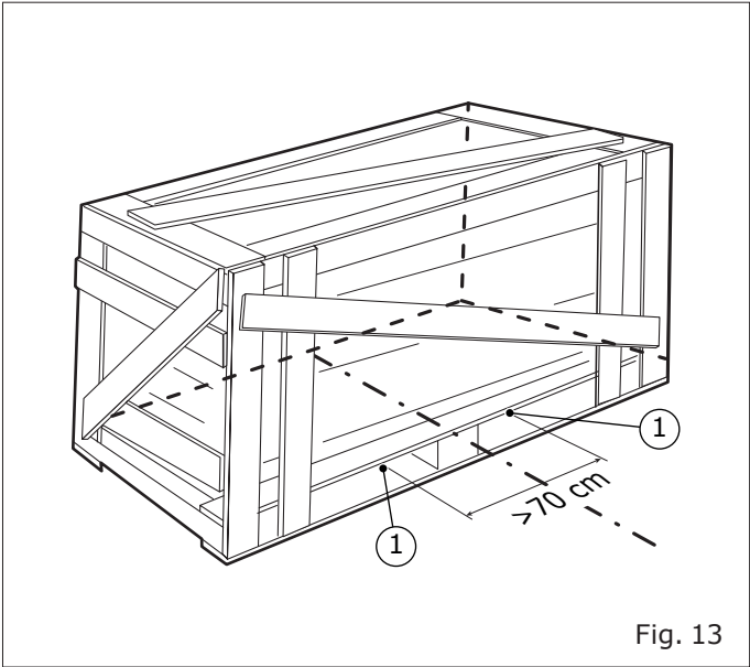
1. Lifting points
