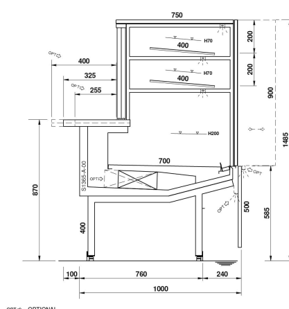
Tower 1500 M
