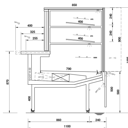
Tower 1500 L
