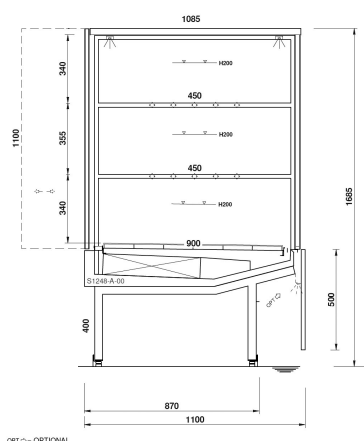
Maturation Tower
