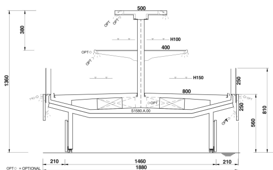
TWIN SV H1400 - LINEAR - 1 SHELF - FRONT 250
