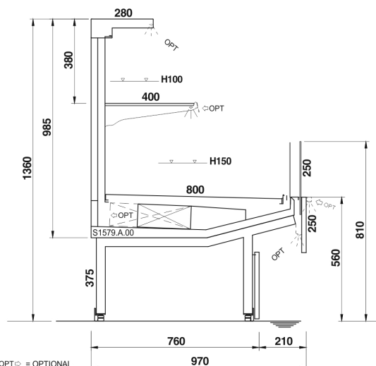
TWIN SV H1400 - EOL - 1 SHELF - FRONT 250
