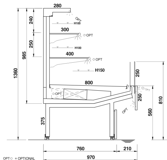
TWIN SV H1400 - EOL - 2 SHELVES - FRONT 250
