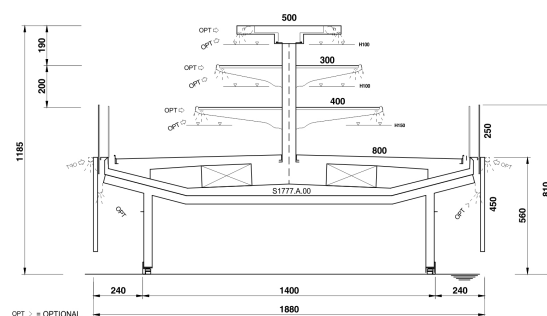
TWIN SV H1200 - LINEAR - 2 SHELVES
