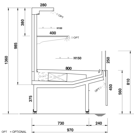
TWIN SV H1400 - EOL - 1 SHELF - FRONT 450
