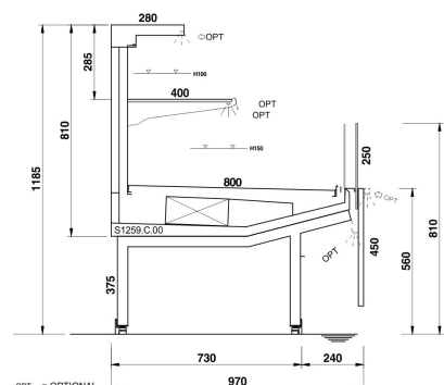
TWIN SV H1200 - EOL - 1 SHELF
