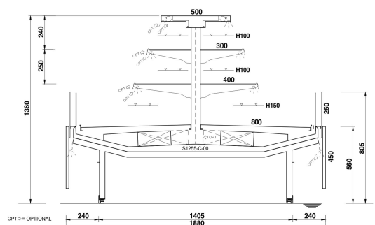
TWIN SV H1400 - LINEAR - 2 SHELVES - FRONT 450
