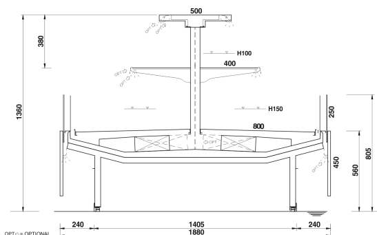
TWIN SV H1400 - LINEAR - 1 SHELF - FRONT 450
