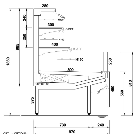
TWIN SV H1400 - EOL - 2 SHELVES - FRONT 450
