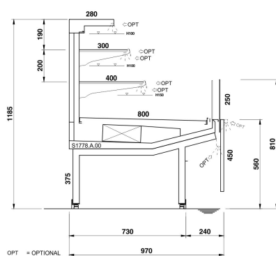
TWIN SV H1200 - EOL - 2 SHELVES
