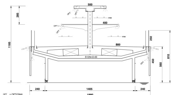
TWIN SV H1200 - LINEAR CABINETS - 1 SHELF
