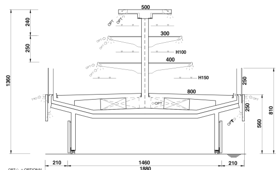
TWIN SV H1400 - LINEAR - 2 SHELVES - FRONT 250
